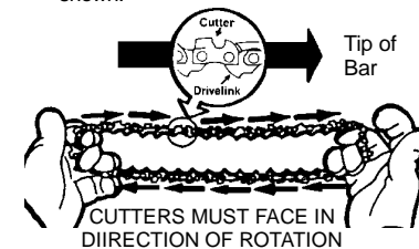
Mount the Bar
